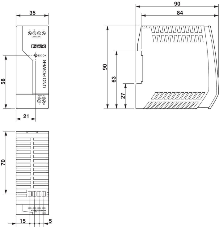
Figure 5 Device dimensions
