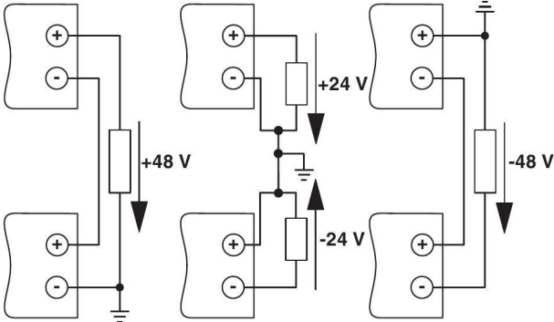
Figure 17 Series operation
